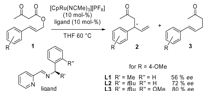
Scheme 2. CpRu-catalyzed rearrangement of primary esters with ligands L .
