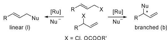
Scheme 1. Allylic substitution of unsymmetrical substrates.
