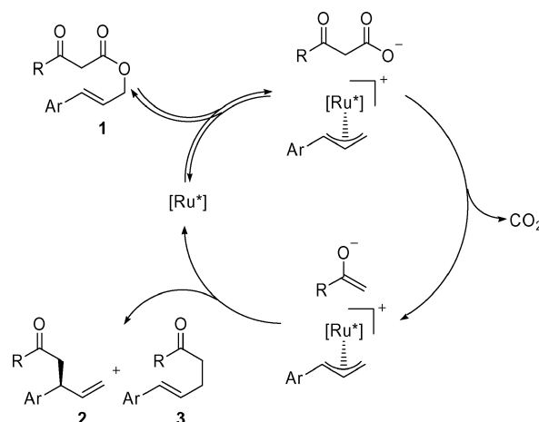
Scheme 4. Postulated mechanistic rationale.
