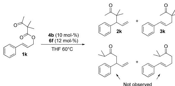
Scheme 6. Conservation of the enolate regiochemistry for 1k .
