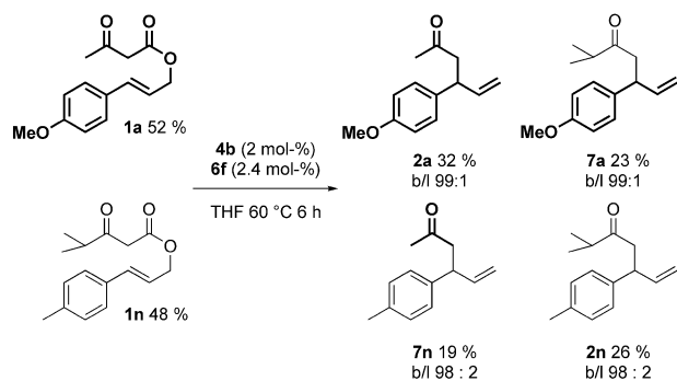
Scheme 5. Double-crossover experiment (linear products 3 and linear crossover products 8 are omitted for clarity; ratios were measured by GC-MS).
