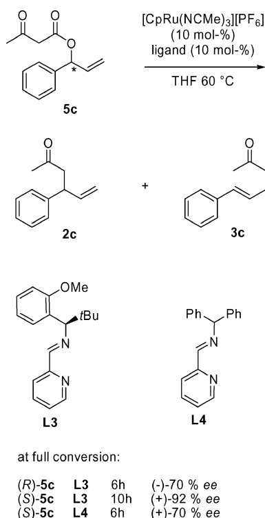
Scheme 3. CpRu-catalyzed rearrangement of secondary esters with ligands L .
